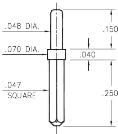
0600-0-05-XX-00-00-01-0 Solder mount in .052 mounting hole
